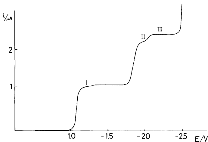
Fig. 4. D.C. polarographic pattern for TCC-PDMS + BF 4 - ( c \cdot 10^{-3} M in DMSO 0.1 M TBAP at 21°C).
