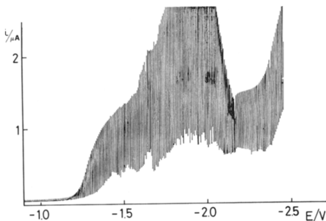
Fig. 1. D.C. polarogram of \text{PDMS}^+ \text{BF}_4^- ( c \cdot 10^{-3} M in DMSO 0.1 M TBAP at 21°C).
