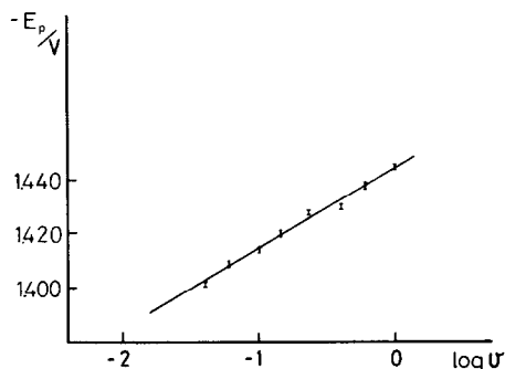
Fig. 3. Sweep rate dependence of the peak potential for the cathodic peak of \text{PDMS}^+ \text{BF}_4^- ( c \approx 2 \times 10^{-3} \text{ M} in DMSO 0.2 M TBAP at 21^\circ\text{C} ).
