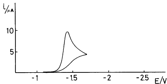
Fig. 2. Potential sweep voltammetry of \text{PDMS}^+ \text{BF}_4^- ( c \approx 2 \times 10^{-3} \text{ M} in DMSO 0.2 M TBAP at 21^\circ\text{C} , v 150 \text{ mV s}^{-1} ).
