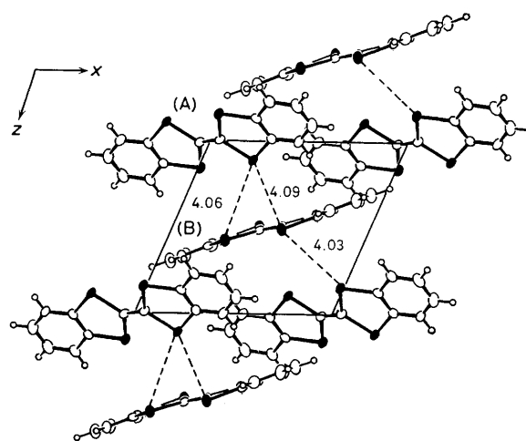
Figure 1. The (010) projection of the crystal structure of DBTSF (7). The molecule labelled A is centred at (0,0,0), while molecule B is centred at (1/2,0,1/2). Se atoms are shaded and closest Se...Se contacts (A) are indicated.
