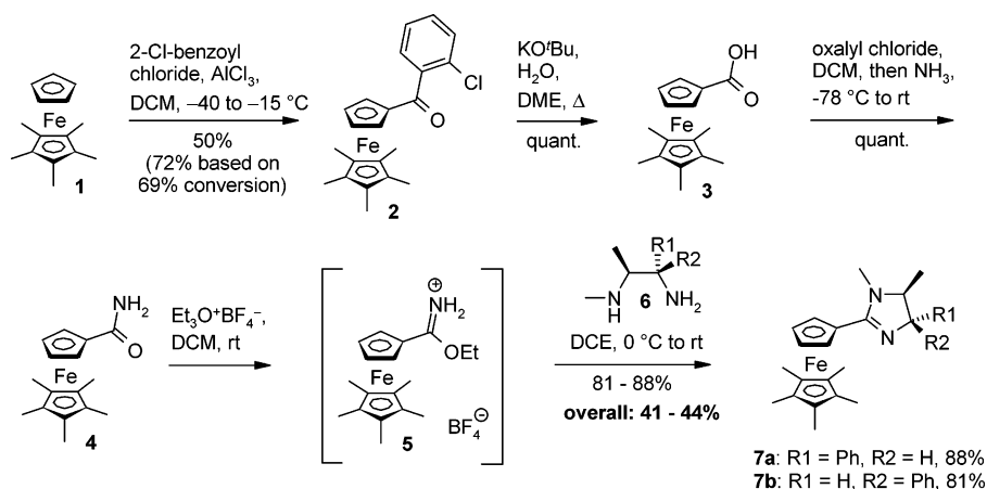
Scheme 2. Synthesis of 1',2',3',4',5'-Pentaphenylferrocene Imidazolines 11
