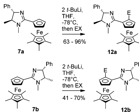
Scheme 3. Diastereoselective ortho -Functionalization of 1',2',3',4',5'-Pentamethylferrocene Imidazolines
