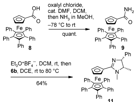
Scheme 2. Synthesis of 1',2',3',4',5'-Pentaphenylferrocene Imidazolines 11
