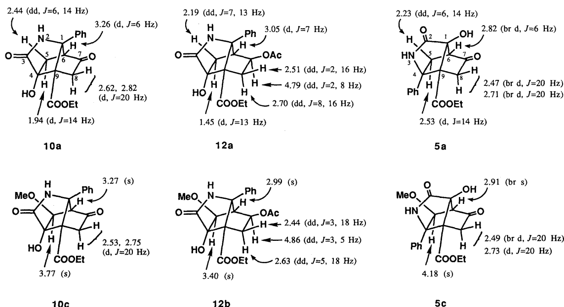
Fig. 1. ^1\text{H} -NMR Data for Azabicyclo[4.3.0.0 4,9 ]nonanes 5a , 5c , 10a , 10c , 12a , and 12b
