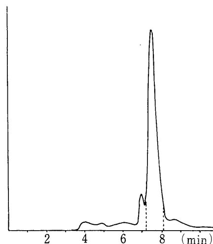
Fig. 2. High-pressure Liquid Chromatography of the Deblocked Pentamer G-U-C-G-G (3) on a Column ( 0.4 \times 25 cm) of C-18 Alkylsilica
