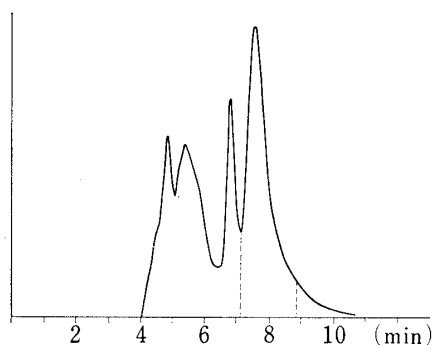
Fig. 4. High-pressure Liquid Chromatography of the Octamer G-U-C-G-U-C-G-G
