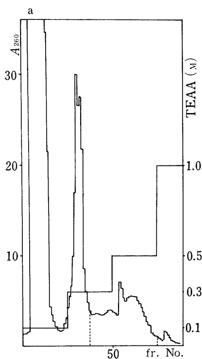
Fig. 3-a. Chromatography of the Reaction Mixture for the Synthesis of the Hexamer on a Column ( 2.5 \times 14 cm) of TEAE-cellulose (Acetate)
