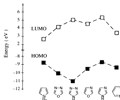
Figure 1. Comparison of HOMO and LUMO energy levels based on ab initio calculations at RHF/6–31G* level of theory.
