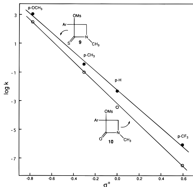
Figure 1. A plot of \log k for solvolyses of mesylates 9 and triflates 10 in trifluoroethanol at 25.0 °C vs \sigma^+ .
