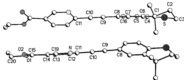
Figure 3. Two selected views of the molecule showing the two moieties of nearly coplanar atoms.
