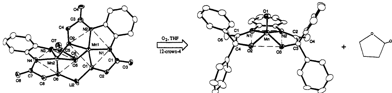
Figure 1. Reaction of 1 with O_2 in THF yields 2 equiv of [Mn^V(O)(PHAB)]^- ( 2 ) 7 and 2-hydroxytetrahydrofuran (THF-OH). On the left is shown an ORTEP drawing of the core of Li_2[Mn^{III}(PHAB)]_2 \cdot 4MeCN for compound 1 , showing the 50% thermal probability ellipsoids. Solvate molecules, hydrogen atoms, and phenyl groups are omitted for clarity. Selected bond distances (Å) and angles (deg) are as follows: Mn1...Mn2, 3.052(9); Mn1-O1, 1.904(5); Mn1-O2, 1.927(5); Mn1-N1, 1.914(6); Mn1-N2, 1.900(5); Mn1-O5, 2.174(5); Mn2-O5, 1.926(5); Mn2-O6, 1.891(5); Mn2-O2, 2.115(5); Mn2-N3, 1.911(6); Mn2-N4, 1.925(6); Li2-O1, 1.87(1); Li2-O6, 1.87(1); Mn1-O2-Mn2, 97.0(2); Mn1-O5-Mn2, 96.0(2); O2-Mn1-O5, 80.3(2); O2-Mn2-O5, 81.9(2); O1-Li2-O6, 113.0(7). On the right side is shown an ORTEP drawing of [Mn^V(O)(PHAB)]^- anion of 2 , showing the 50% thermal probability ellipsoids. Hydrogen atoms are omitted for clarity. Selected bond distances (Å) and angles (deg) are as follows: Mn-O1, 1.558(4); Mn-O2, 1.827(4); Mn-O3, 1.831(4); Mn-N1, 1.893(5); Mn-N2, 1.875(5); O1-Mn-O2, 110.0(2); O1-Mn-O3, 110.0(2); O1-Mn-N1, 109.2(2); O1-Mn-N2, 108.5(2).
