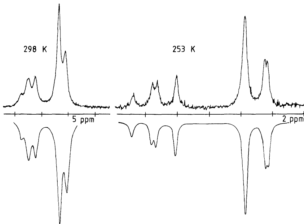
Fig. 2. 109 MHz (^1H) ^{31}P NMR spectra of Vb measured at 298 and 253 K (top) and calculated (bottom) using the parameters given in the experimental part. Half width ca. 100 Hz at 298 K, ca. 27 Hz at 253 K.
