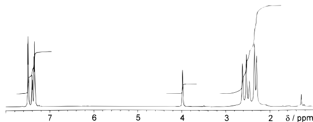
Figure 9. 1 H{ 11 B} NMR spectrum of 1.
