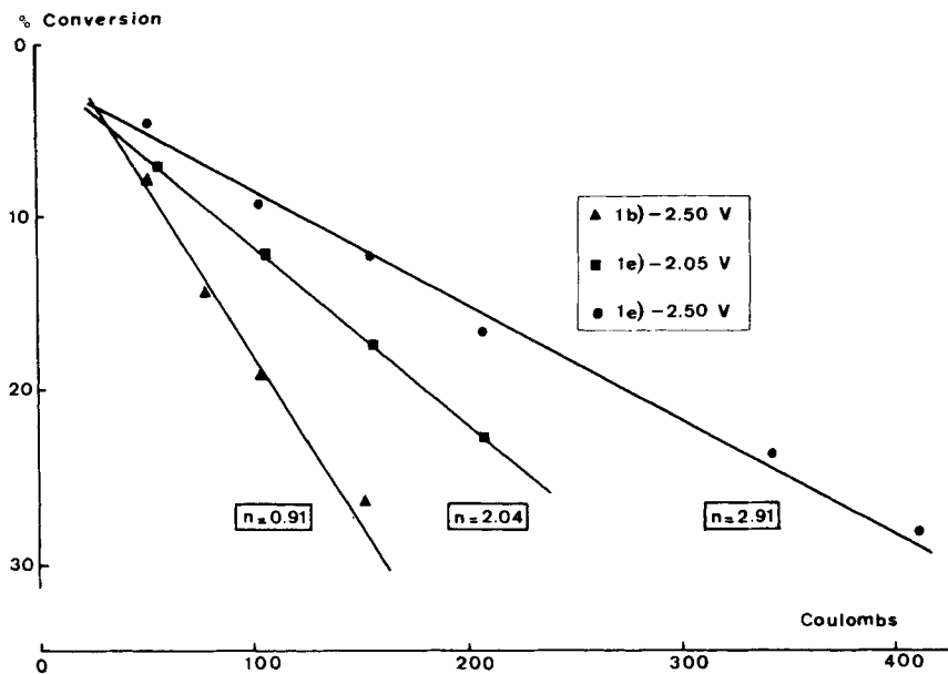
Fig. 2. Current quantity vs. conversion of starting material. Reference electrode: \text{Ag}/\text{Ag}^+
