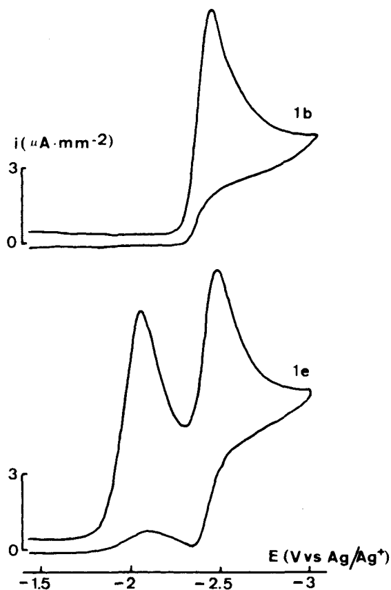
Fig. 1. Cyclic voltammogram of 1b and 1e ( 10^{-3} M in \text{CH}_3\text{CN} ). Scan rate = 500 \text{ mV} \cdot \text{sec}^{-1}
