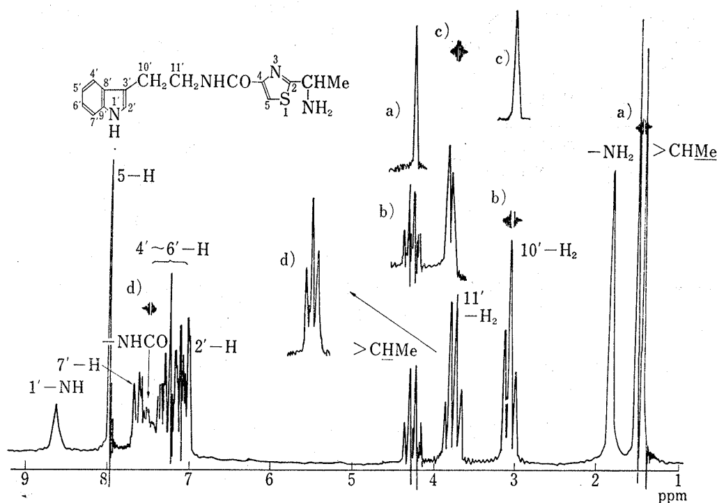
Fig. 1. NMR Spectrum of 1 (CDCl 3 , 100 MHz)
