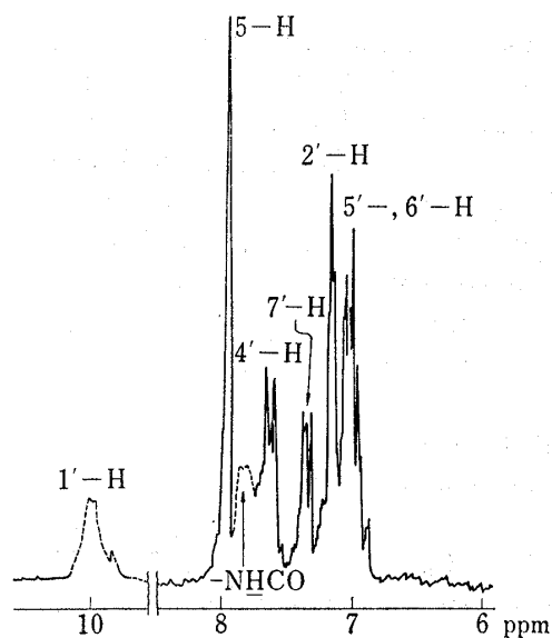
Fig. 2. NMR Spectrum of 1 (100 MHz, Acetone- d 6 )
