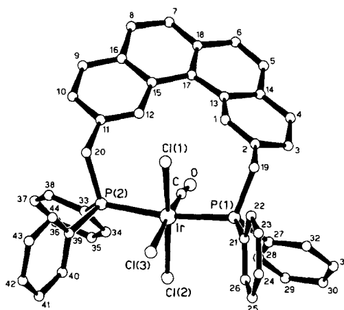
Fig. 2. A computer-generated drawing of the molecule [\text{IrCl}_3(\text{CO})(\mathbf{1})]
