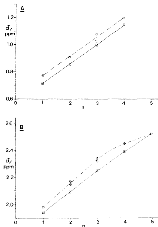
Fig. 2. Variation of the methyl NMR resonances with degree of substitution in [M(CO)_{5-n}(CNR)_nBr] complexes. (A) \odot = [Mn(CO)_{5-n}(CNBu-t)_nBr] , \square = [Re(CO)_{5-n}(CNBu-t)_nBr] . (B) \odot = [Mn(CO)_{5-n}(CNC_6H_3Me_2-2,6)_nBr] , \square = [Re(CO)_{5-n}(CNC_6H_3Me_2-2,6)_nBr] .
