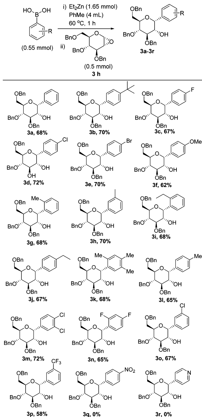
Scheme 1. Substrate Scope of Arylboronic Acids for \alpha -Arylation with Glucal Epoxide
