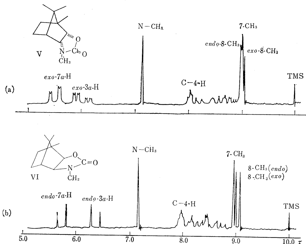
Fig. 1. The Nuclear Magnetic Resonance Spectra of V and VI in Deuteriochloroform
