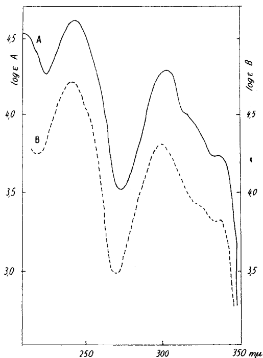
Fig. 3. 7-Oxy-yobyrin (A) Harmol (B)
