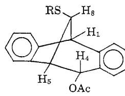
VIIIa, R = C 6 H 5 b, R = CH 3
