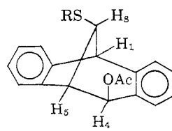
VIIa, R = C 6 H 5 b, R = CH 3
