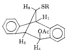
Va, R = C 6 H 5 b, R = CH 3
