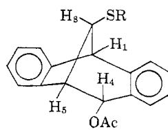
VIa, R = C 6 H 5 b, R = CH 3
