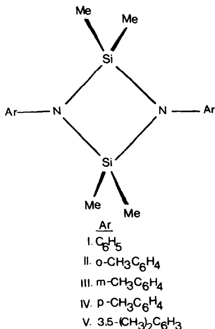
Fig. 1. The structural formula of tetramethyl- N,N' -diarylcyclodisilazanes.
