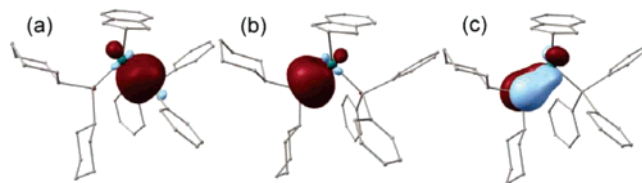
Figure 3. Occupied natural orbitals relevant to Ru–P bonds resulting from NBO analysis of the calculated structure of 2a : (a) Ru– \text{PPh}_3 \sigma ; (b) Ru– \text{PCy}_2 \sigma ; (c) Ru– \text{PCy}_2 \pi .
