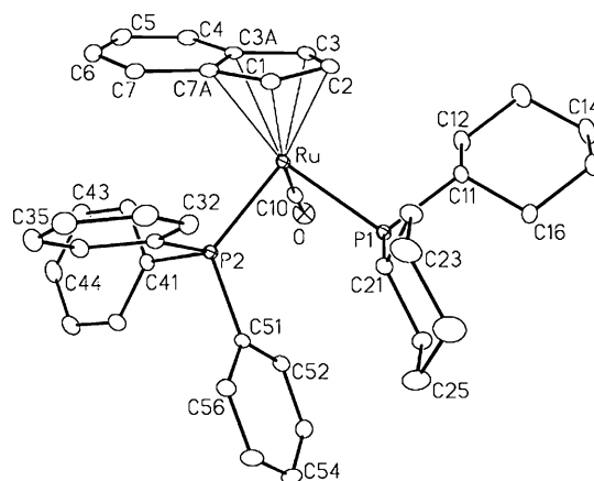
Figure 4. Molecular structure of [\text{Ru}(\text{PCy}_2)(\eta^5\text{-indenyl})(\text{CO})(\text{PPh}_3)] ( 3a ). Selected interatomic distances (Å) and bond angles (deg): Ru–P(1) = 2.4390(7), Ru–P(2) = 2.3158(6), Ru–C* = 1.973, \Delta = 0.154 ; P(1)–Ru–P(2) = 90.92(2), P(1)–Ru–C* = 125.8, P(2)–Ru–C* = 125.4, Ru–P(1)–C(11) = 107.36(8), Ru–P(1)–C(21) = 107.88(8), C(11)–P(1)–C(21) = 102.47(10).
