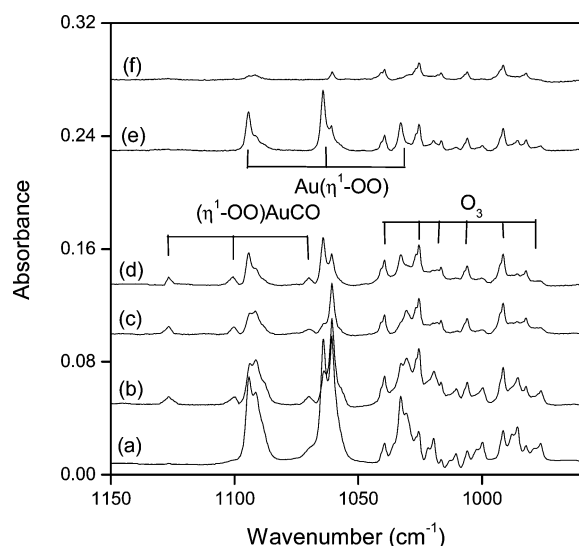
Figure 9. Infrared spectra in the 1150–960 \text{cm}^{-1} region from co-deposition of laser-ablated Au atoms with 0.5% CO + 3.5% ^{16}\text{O}_2 + 7.0% ^{16}\text{O}^{18}\text{O} + 3.5% ^{18}\text{O}_2 in Ar: (a) 1 h of sample deposition at 7 K; (b) after annealing to 25 K; (c) after annealing to 30 K; (d) after 20 min of \lambda > 340 nm irradiation; (e) after 20 min of broad-band irradiation; (f) after annealing to 34 K.
