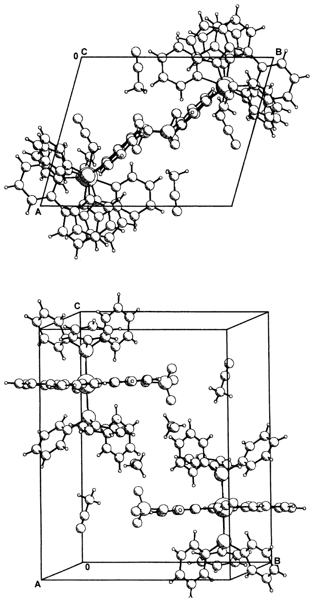
Fig. 3. Top: 2-D packing diagram of [\text{Ru}(\text{tpy})(\text{PPh}_3)_2(\text{N}_3)]^+[\text{ClO}_4]^- (PLUTO representation) [20]. Bottom: 3-D packing diagram of [\text{Ru}(\text{tpy})(\text{PPh}_3)_2(\text{N}_3)]^+[\text{ClO}_4]^- (PLUTO representation) [20].
