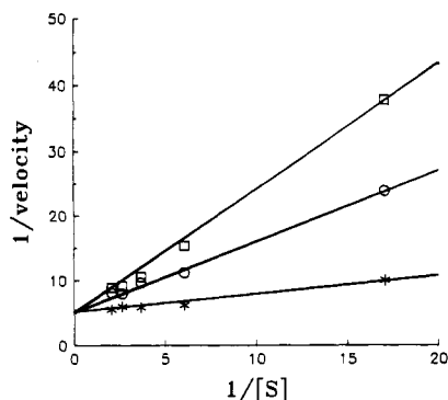
Figure 1. Double reciprocal plot of aromatase inhibition by inhibitor 8. Varying concentrations of androstenedione were incubated with aromatase at single inhibitor concentrations of 0 \mu M (*), 0.3 \mu M (O), or 0.6 \mu M ( \square ). Each point represents the average of two determinations with a variation of less than 7%.
