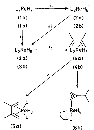
Scheme 1. Postulated reaction paths. For (a), L = PPh_3 and (b), L_2 = Ph_3PCH_2CH_2PPh_2 . Reagents: i, L = PPh_3 , THF, 65 °C, -H_2 ; ii, Bu^tOK , -Bu^tOH ; iii, Me_2SO_4 , -CH_4 ; iv, 2,3-dimethylbutadiene. Species ( 3 ) and ( 4 ) are postulated intermediates which have not been isolated or characterised.
