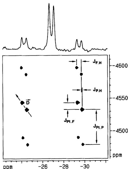
Fig. 2. Part of the conventional ^1\text{H} spectrum and the contour plot of the ^{195}\text{Pt} – ^1\text{H} heteronuclear correlation (5.9 Tesla) for \text{trans-}[\text{PtH}(\text{F})\text{PCy}_3]_2 recorded in toluene- d_8 . The orientation of the displacement vector D results from unlike signs of ^1J(^{195}\text{Pt}, ^{19}\text{F}) and ^2J(^{19}\text{F}, ^1\text{H}) .
