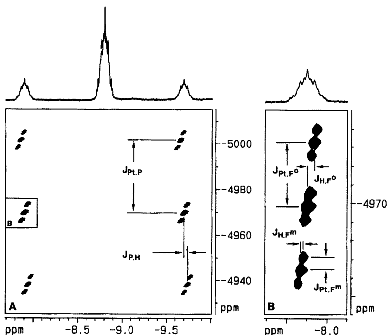
Fig. 1. ^{195}\text{Pt} - ^1\text{H} heteronuclear correlation (9.4 Tesla) for \text{trans-}[\text{PtH}(\text{C}_6\text{F}_4\text{CN})(\text{PCy}_3)_2] recorded in \text{CDCl}_3 showing in \omega_1 the t \times t \times t multiplicity due to two ^{31}\text{P} spins (A) and F_{\text{ortho}} and F_{\text{meta}} (B). The hydride region of a conventional ^1\text{H} spectrum is shown above the contour maps.
