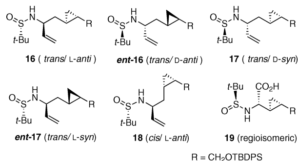
Fig. 5 The key methanoamino acid equivalents for the synthesis of belactosin A and its stereo- and regioisomers.
