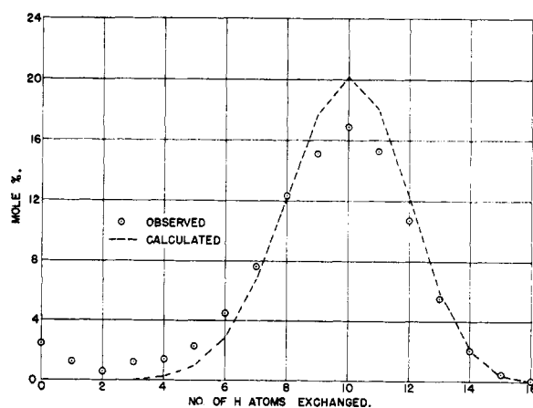
Fig. 1.—Exchange of 2-methylhexane and deuterated catalyst; comparison of observed distribution of products with that calculated assuming statistical distribution.
