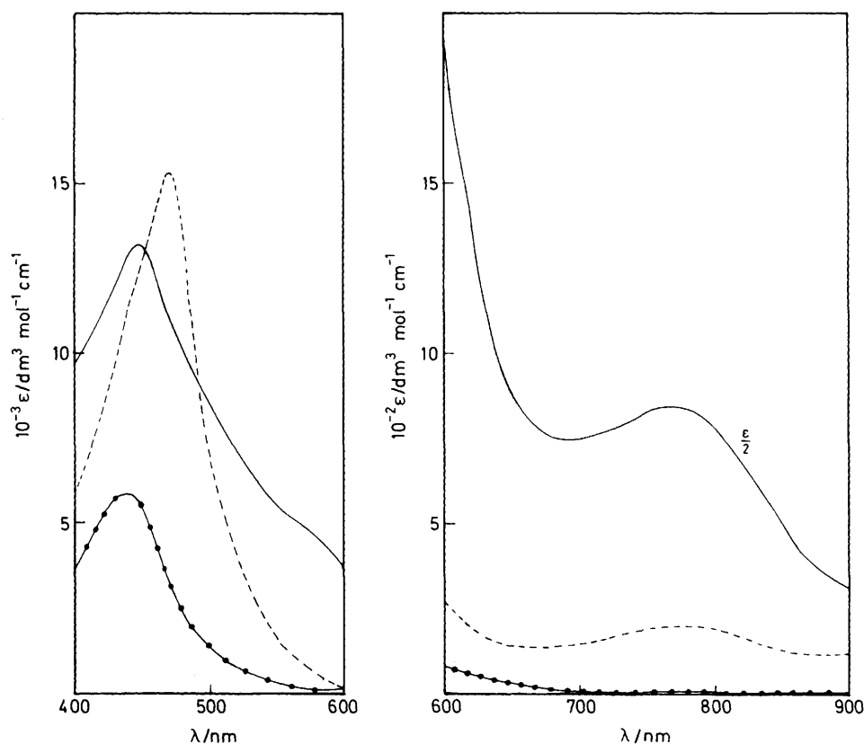
Figure 1. Electronic spectra of [\text{Cu}_2(\text{HL})_2(\text{L})_2] (1) (—) (in benzene), [\text{CuL}(\text{PPh}_3)_2] (2a) (---) (in acetone), and [\text{Cu}(\text{HL})(\text{PPh}_3)_2(\text{ClO}_4)] (5) (- · - · -) (in methanol)
