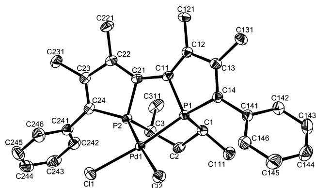
Figure 9. Molecular view of R[Rp,Sp,Sc,Sc]-\mathbf{15} with atom-labeling scheme. Ellipsoids represent 50% probability. Selected bond distances (Å): \text{Pd}(1)-\text{P}(1) 2.2735(6); \text{Pd}(1)-\text{P}(2) 2.2479(6); \text{Pd}(1)-\text{Cl}(1) 2.3381(7); \text{Pd}(1)-\text{Cl}(2) 2.3514(6); \text{P}(1)-\text{C}(1) 1.867(3); \text{P}(1)-\text{C}(11) 1.820(2); \text{P}(1)-\text{C}(14) 1.803(3); \text{P}(2)-\text{C}(3) 1.845(3); \text{P}(2)-\text{C}(21) 1.803(3); \text{P}(2)-\text{C}(24) 1.796(3).
