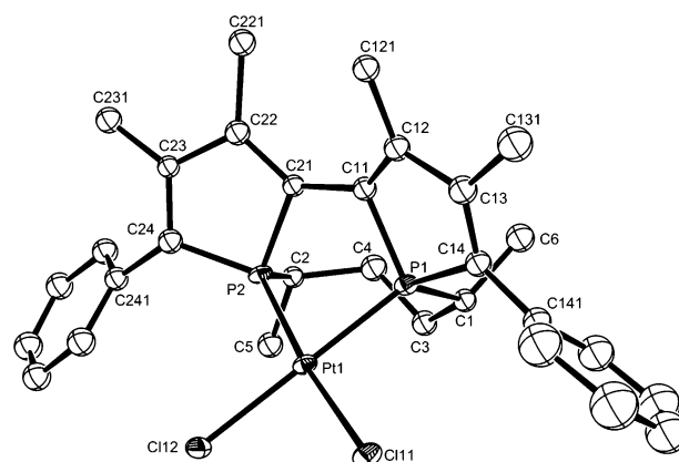
Figure 10. Molecular view of S[Rp,Sp,Rc,Rc]-\mathbf{17} with atom-labeling scheme. Ellipsoids represent 30% probability. Selected bond distances (Å): \text{Pt}(1)-\text{P}(1) 2.239(4); \text{Pt}(1)-\text{P}(2) 2.247(4); \text{Pt}(1)-\text{Cl}(1) 2.348(4); \text{Pt}(1)-\text{Cl}(2) 2.350(4); \text{P}(1)-\text{C}(1) 1.80(2); \text{P}(1)-\text{C}(11) 1.82(2); \text{P}(1)-\text{C}(14) 1.78(2); \text{P}(2)-\text{C}(2) 1.87(2); \text{P}(2)-\text{C}(21) 1.82(2); \text{P}(2)-\text{C}(24) 1.77(2).
