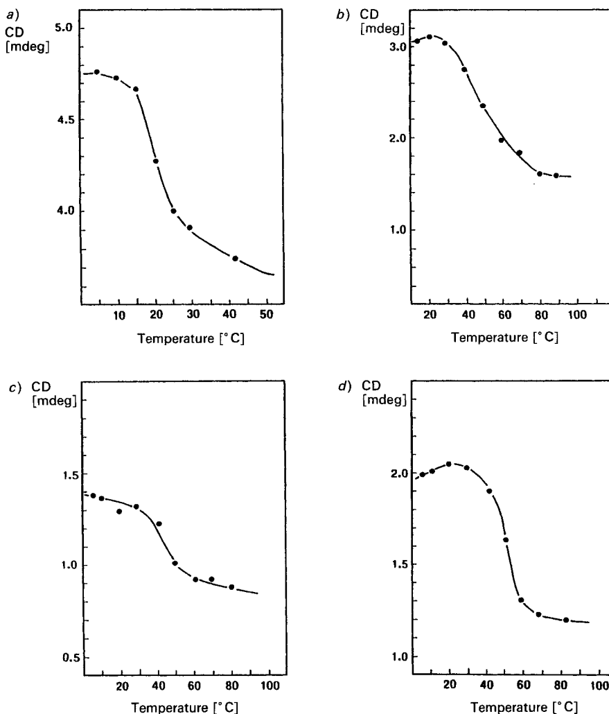
Fig. 2. Temperature-dependent CD spectra (CD vs. temp.; B_{2u} transition) of a) d(c^3A-T)_6 ( 14 ), b) d(A-T)_6 ( 15 ), c) d(G-T-A-G-c^3A-c^3A-T-T-C-T-A-C) ( 16 ), and d) d(G-T-A-G-A-A-T-T-C-T-A-C) ( 18 ). In 60 mM Na cacodylate buffer (pH 7.0), 1M NaCl, and 100 mM MgCl_2 ( 3.0 \mu M single-strand concentration).
