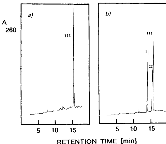
Fig. 3. HPLC profiles of the reaction mixture from the cleavage of d(G-T-A-G- c^3A - c^3A -T-T-C-T-A-C) ( 16 ) by the endodeoxyribonuclease EcoRI (conditions, see Exper. Part ; solvent system IV) a) at the beginning and b) after 101 min. I, d(G-T-A-G); II, d( pc^3A - c^3A -T-T-C-T-A-C); III, dodecanucleotide 16 .
