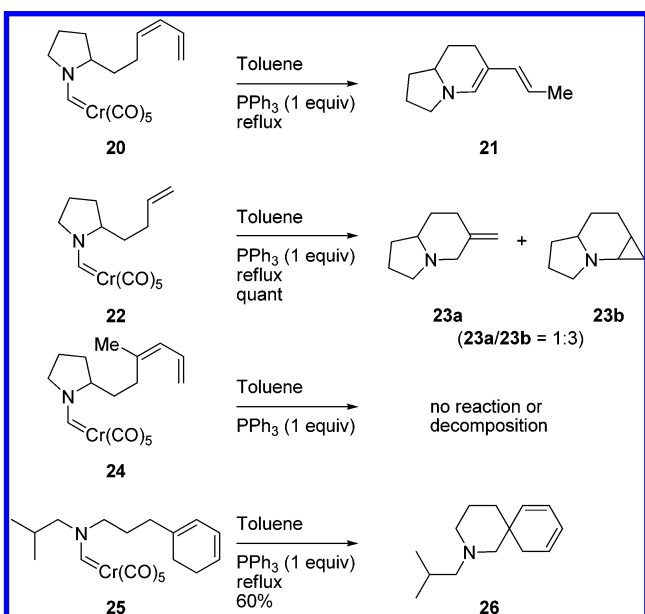
Scheme 5. Reactions of CAMC 20 , 22 , 24 , and 25
