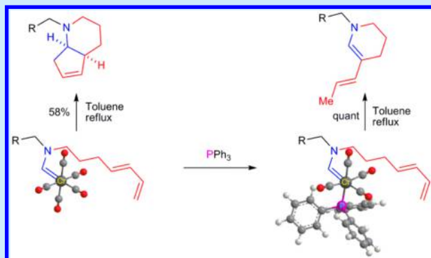
Scheme 2. Main Methods of Preparation of CAMC
