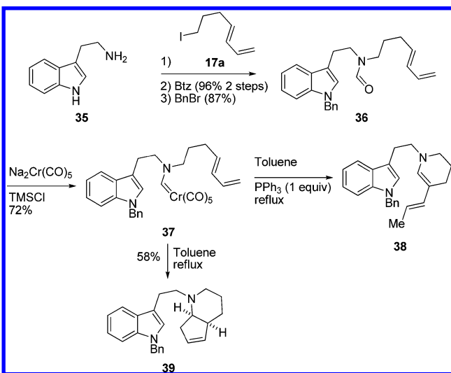
Scheme 8. Alkaloid-like Structures via Reaction of CAMC 37
