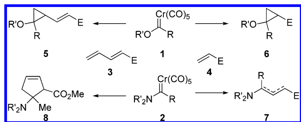
Scheme 1. Reactions of CALC 1 and CAMC 2
