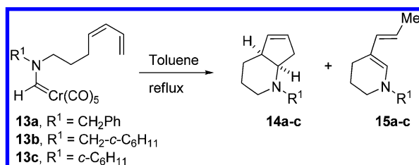
Scheme 3. Formal [4 + 1] -Cycloaddition and \beta -Hydride Elimination of CAMC 13a–c Tethered to a Diene
