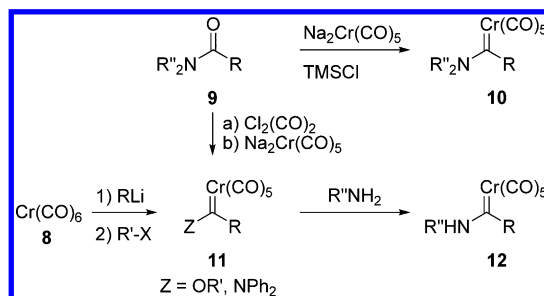
Scheme 2. Main Methods of Preparation of CAMC
