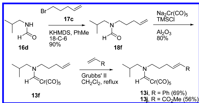
Scheme 4. Synthesis of CAMC 13f and 13i–j
