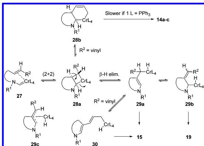
Scheme 6. Plausible Mechanism for the Formation of Products 15 and 19
