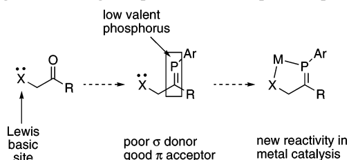
Scheme 1. Strategy for the Preparation of Phosphaalkene Ligands Bearing Unique Donor–Acceptor Properties
