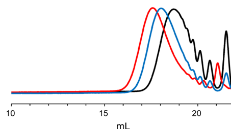
Figure 2. SEC curves (RI) obtained by the first polymerization of 1 (polymer 2 , black) and sequential addition of 1 (polymer 2' , blue) and 7 (polymer 8 , red) after the first polymerization of 1 .
