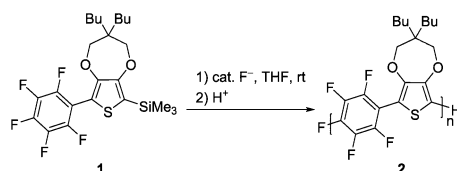
Scheme 1. Polymerization of 1
