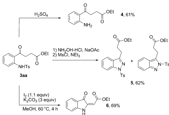
Scheme 3. Derivatization of a hydroacylation product.
