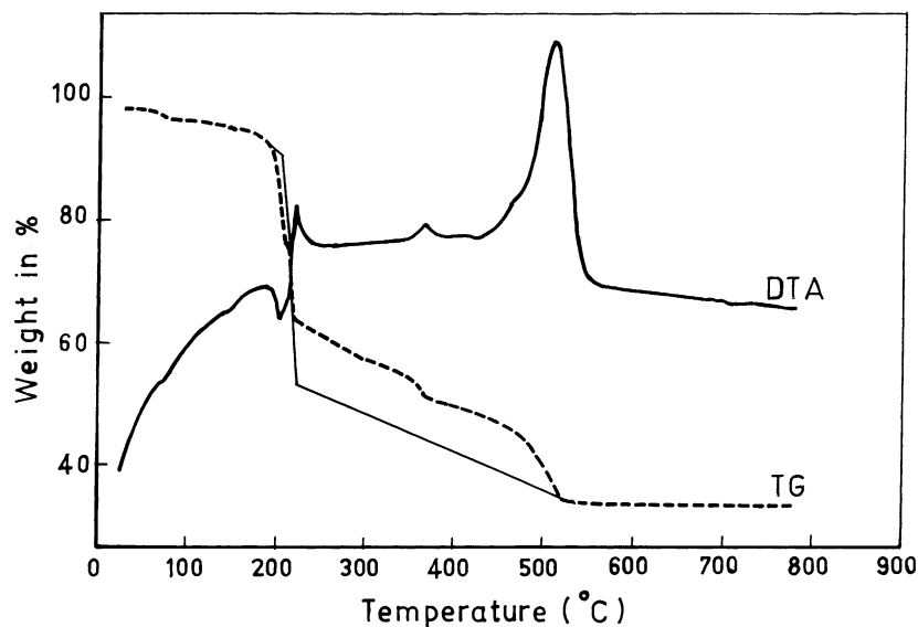
Fig. 2. TG–DTA of the complex (Tb 5 ).
