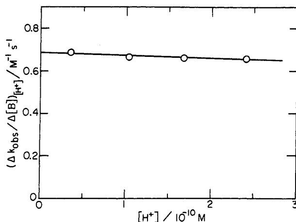
Figure 4. Relationship between (\Delta k_{\text{obs}}/\Delta[B])_{[H^+]} and [H^+] for the decomposition of nitramide in \text{CH}_3\text{OCH}_2\text{CH}_2\text{CH}_2\text{NH}_3^+ / \text{CH}_3\text{OCH}_2\text{CH}_2\text{CH}_2\text{NH}_2 buffer solutions at 25 °C, ionic strength = 0.1 M.
