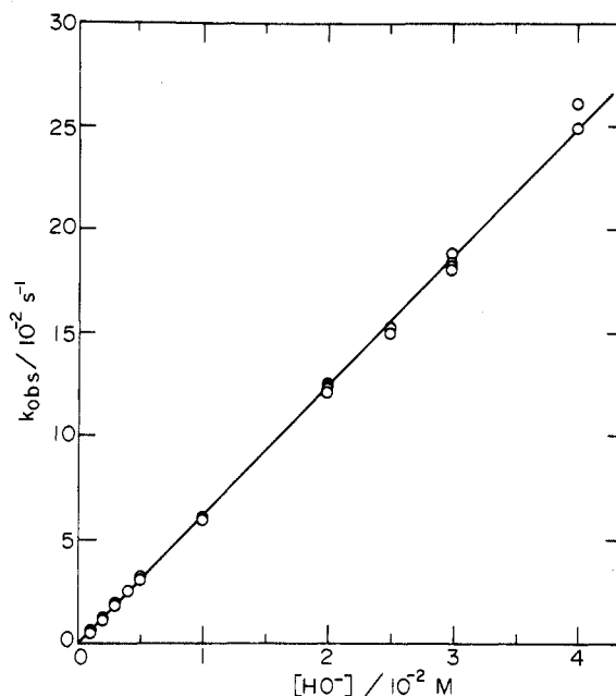
Figure 1. Relationship between rates of nitramide decomposition and hydroxide ion concentration in aqueous solution at 25^\circ\text{C} , ionic strength = 0.1\text{ M} .
