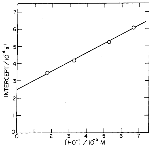
Figure 5. Relationship between hydroxide ion concentration and intercepts of buffer dilution plots for the decomposition of nitramide in \text{HCN}/\text{CN}^- buffer solutions at 25 °C, ionic strength = 0.1 M.
