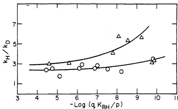
Figure 7. Kinetic isotope effects on the base-catalyzed decomposition of nitramide in aqueous solution at 25 °C: (O) oxygen bases and (Δ) nitrogen bases.
