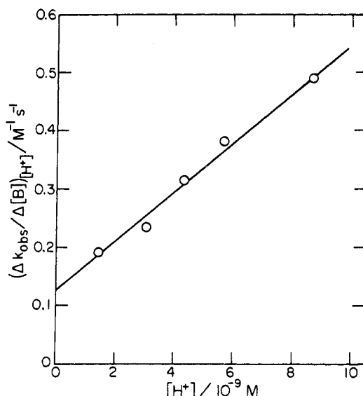
Figure 3. Relationship between (\Delta k_{\text{obs}}/\Delta[B])_{[H^+]} and [H^+] for the decomposition of nitramide in (\text{CH}_3\text{O})_2\text{CHCH}_2\text{NH}_3^+ / (\text{CH}_3\text{O})_2\text{CHCH}_2\text{NH}_2 buffer solutions at 25 °C, ionic strength = 0.1 M.
