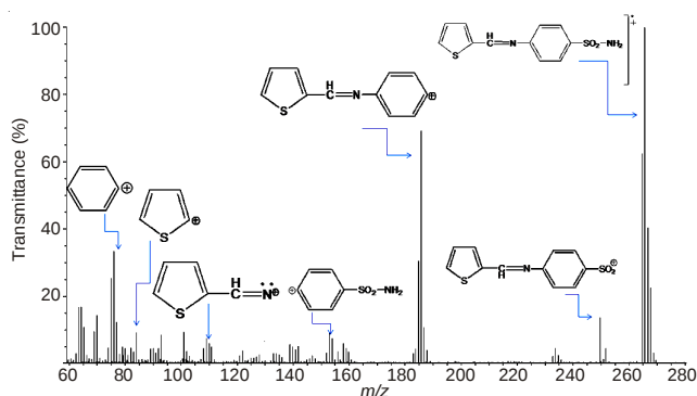
Fig. 2. Mass spectrum of the ligand
