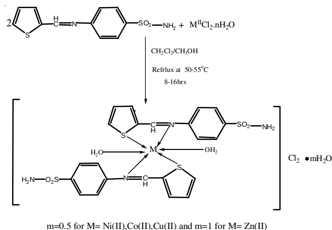
Fig. 4. General scheme for the synthesis of M(II) complexes
