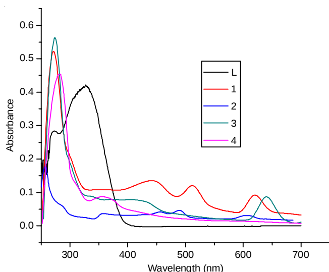
Fig. 5. Electronic absorption spectra of L and its complexes
