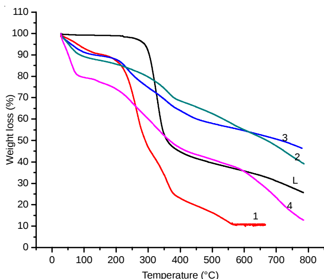
Fig. 6. Thermograms of L and its metal complexes
