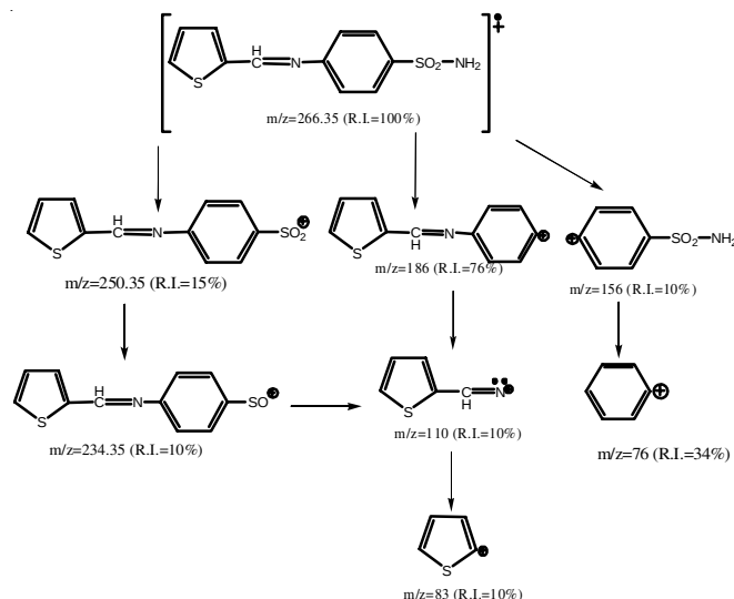
Fig. 3. Suggested mass fragmentation of the ligand
