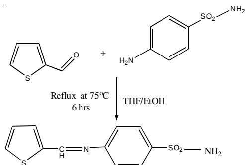
Fig. 1. General scheme for the synthesis of Schiff base (L)
