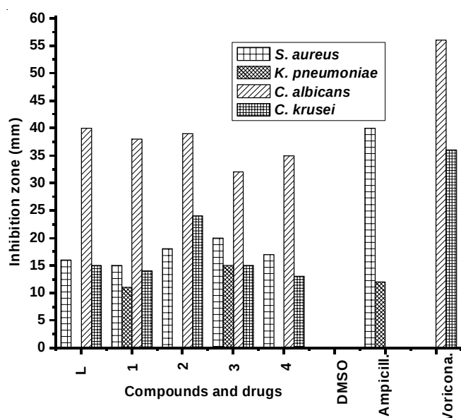
Fig. 7. Zone of inhibitions of reported compounds and standards against four types of microorganisms (two bacteria and two fungi)
