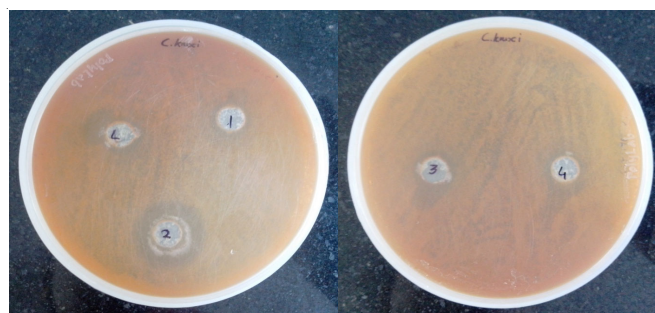
Fig. 8. Photograph showing antifungal studies of L and its metal complexes against C. krusei
