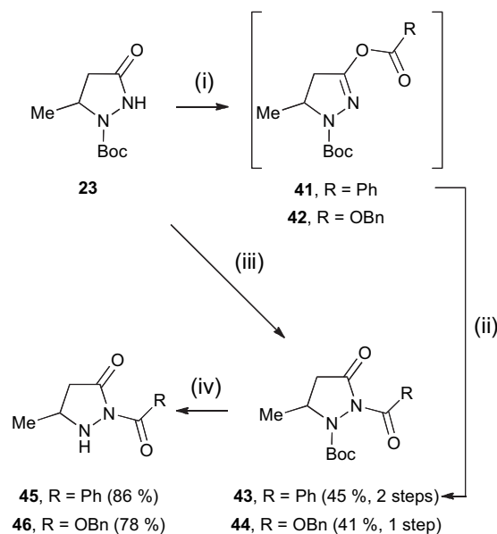
Scheme 4. Reagents and conditions: (i) \text{NEt}_3 , \text{CH}_2\text{Cl}_2 , then benzoyl chloride or benzyl chloroformate, -78^\circ\text{C} to rt; (ii) toluene, reflux; (iii) NaH, \text{CH}_2\text{Cl}_2 , then benzyl chloroformate, -78^\circ\text{C} to rt; (iv) TFA, \text{CH}_2\text{Cl}_2 , rt.
