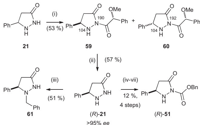
Scheme 8. Reagents and conditions: (i) EDCI·HCl, HOBT, ( R )- O -methyl mandelic acid, DMF; (ii) 5 M HCl (aq), reflux; (iii) benzaldehyde, EtOH, rt, then NaBH 4 . (iv) tert -butyl dicarbonate, Na 2 CO 3 , dioxane/H 2 O, rt; (v) NaH, CH 2 Cl 2 , then benzyl chloroformate, −78 °C to rt; (vi) toluene, reflux; (vii) TFA, CH 2 Cl 2 , rt.
