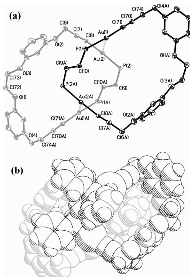
Fig. 1 The structure of complex 3g , [1,2-C 2 H 4 (O-3-C 6 H 4 OCH 2 C≡CAu) 2 (μ- trans -Ph 2 CH=CHPPh 2 )] n , showing the association of two rings through Au...Au bonding: (a) the macrocyclic ring structure and Au...Au bonds (phenyl groups and hydrogen atoms are omitted for clarity); and (b) a space-filling model with all atoms included, illustrating the penetration of a phenyl group through each cavity. Symmetry operations for equivalent atoms: -x + 2 , -y + 1 , -z + 1 .
