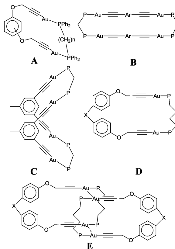
Chart 1 Macroscopic dialkynyl(diphosphine)gold(I) complexes.
