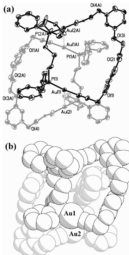
Fig. 2 The molecular structure of complex 3d , [1,2-C 2 H 4 (O-3-C 6 H 4 OCH 2 C≡CAu) 2 (μ-Ph 2 P(CH 2 ) 4 PPh 2 )] 2 , with hydrogen atoms omitted for clarity: (a) the ring structure and intermolecular auriphilic bonding, and (b) a space-filling model showing the phenyl group of one molecule penetrating the cavity of the other. Symmetry operations for equivalent atoms: -x + 1, -y, -z + 1 .
