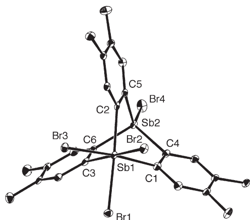
Figure 2. ORTEP drawing of 4 . Hydrogen atoms and \text{CHCl}_3 are omitted for clarity. Selected bond lengths (Å) and angles (°): Sb1–C1, 2.190(3); Sb1–C2, 2.213(3); Sb1–C3, 2.200(3); Sb1–Br1, 2.6691(4); Sb1–Br2, 2.6339(4); Sb1–Br3, 2.6359(4); C1–Sb1–Br1, 173.6(1); C2–Sb1–Br2, 172.0(1); C3–Sb1–Br3, 174.6(1); C1–Sb1–C2, 92.9(1); C1–Sb1–C3, 95.6(1); C2–Sb1–C3, 96.3(1); C4–C1–Sb1, 121.5(2); C5–C2–Sb1, 123.1(2); C6–C3–Sb1, 121.5(2); Sb2–Br4, 2.4066(4); Sb2–C4, 2.096(3); Sb2–C5, 2.086(3); Sb2–C6, 2.080(3); C4–Sb2–C5, 100.5(1); C4–Sb2–C6, 105.0(1); C5–Sb2–C6, 105.7(1); C4–Sb2–Br4, 108.4(1); C5–Sb2–Br4, 116.8(1); C6–Sb2–Br4, 108.4(1); C1–C4–Sb2, 114.8(2); C2–C5–Sb2, 113.2(2); C3–C6–Sb2, 113.4(2); Sb1...Sb2, 3.426.
