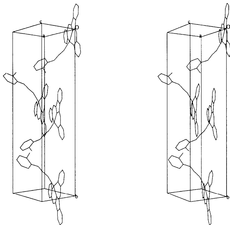
Fig. 2. Stereoview of the unit cell for the complex \text{Ni}(\text{L})(2\text{-Clpcyd}) .
