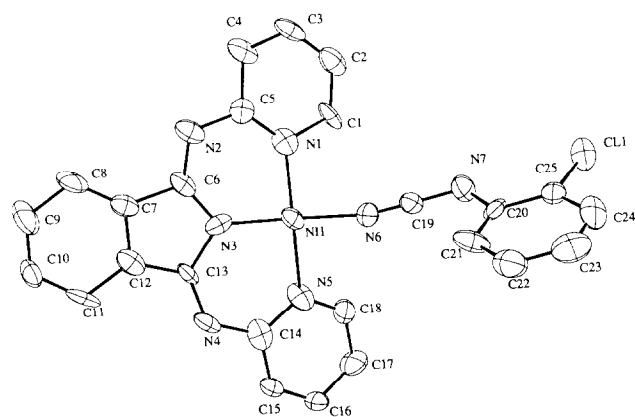
Fig. 1. ORTEP drawing of the complex Ni(L)(2-Clpcyd).
