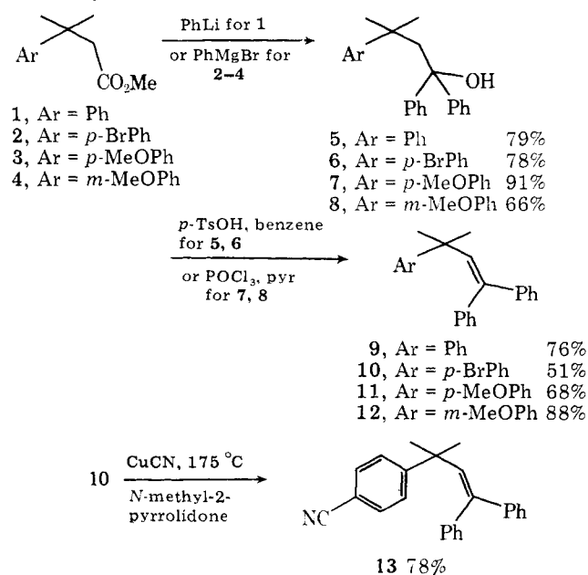
Chart I. Synthesis of Photochemical Reactants
