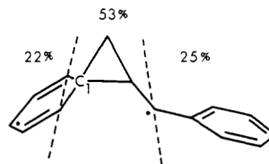
Figure 4. \Delta E_{rt} treatment for the cyclopropyldicarbonyl diradical, excitation energy partitioning.
