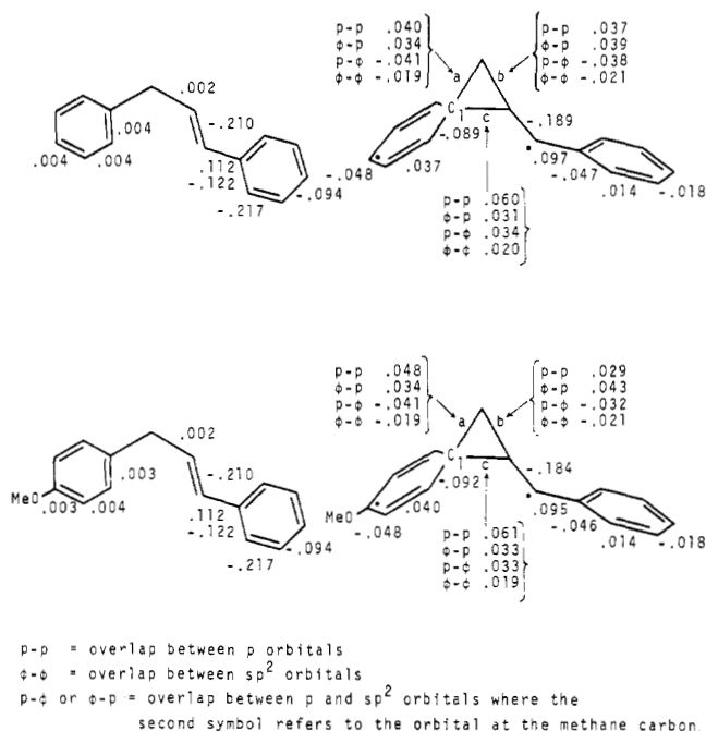
Figure 3. \Delta P_{rt} treatment for aryl vinyl methanes and the derived cyclopropyldicarbonyl diradicals.
