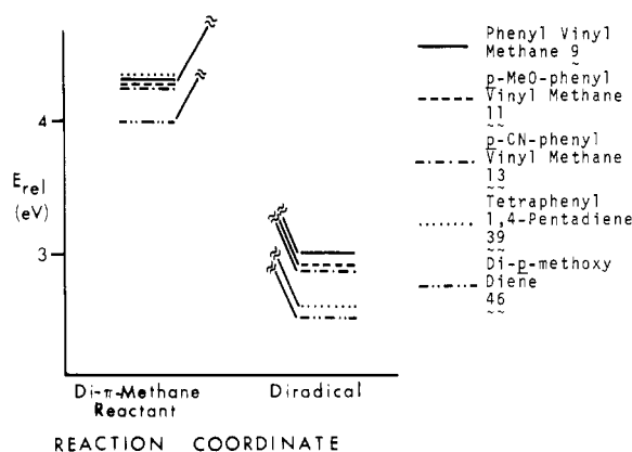
Figure 5. Energetics of bridging.
