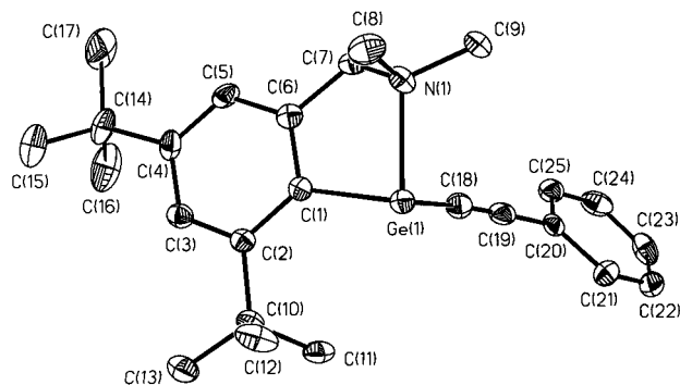
Figure 3. Molecular structure of 6.
