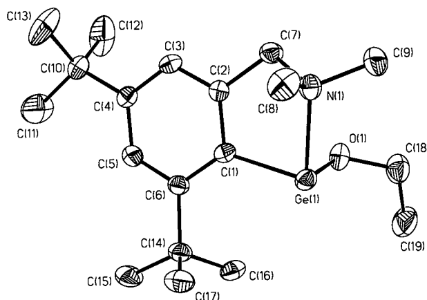
Figure 2. Molecular structure of 4 .
