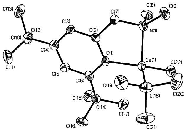
Figure 5. Molecular structure of 11a .
