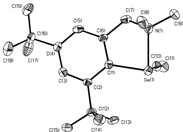
Figure 4. Molecular structure of 7 .
