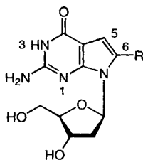
2a R = H
