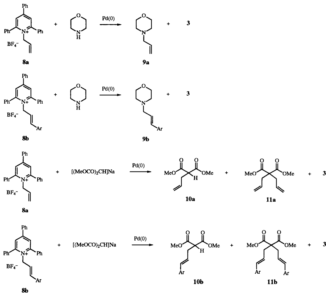
Scheme 4 Pd(0)-Catalyzed reactions of N -allyl-2,4,6-triphenylpyridinium tetrafluoroborates with morpholine and sodium dimethyl malonate.
