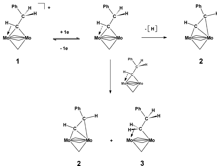
Scheme 4
