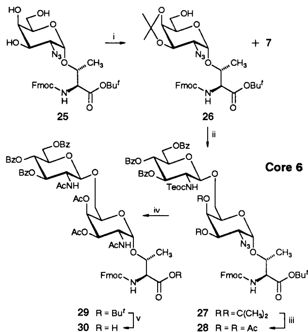
Scheme 3 Reagents: i, (CH 3 ) 2 CH(OCH 3 ) 2 , PTSA; ii, TMSOTf; iii, AcOH, Ac 2 O, Pyr; iv, Zn, Ac 2 O, AcOH, THF; v, TFA (95%)
