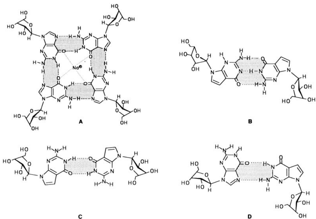
Fig. 2. Tetrameric structure A of U-G-G-G-U ( 8 ) [5], and proposed dimer structures B and C for U-c 7 G-c 7 G-c 7 G-c 7 G-U ( 11 ), and dimer structure D for oligomers containing G and c 7 G, e.g. U-G-c 7 G-G-G-U ( 9 )
