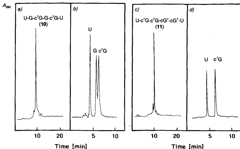
Fig. 1. HPLC Profiles on a RP-18 column of a) c) the crude oligomers 10 or 11 after desilylation and desalting and b) d) after enzymatic hydrolysis of 10 and 11 with snake-venom phosphodiesterase and alkaline phosphatase. For conditions, see Exper. Part .
