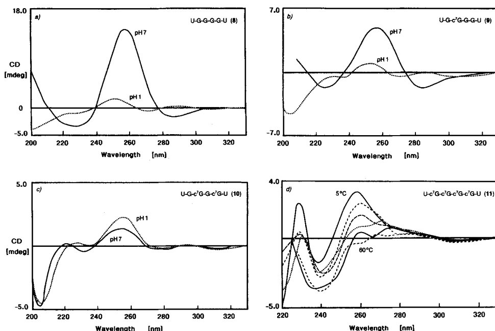
Fig. 4. CD Spectra of a) U-G-G-G-G-U ( 8 ), b) U-G-c 7 G-G-G-U ( 9 ), c) U-G-c 7 G-G-c 7 G-U ( 10 ), and U-c 7 G-c 7 G-c 7 G-c 7 G-U ( 11 ). 0.5 A_{260} units in 0.1M NaCl at pH 1.0 or pH 7.0 at 5°; temperature-dependent CD spectra at pH 7 of 11 at 5° (—), 10° (---), 20° (· · ·), 25° (— · —), 40° (— — —), and 60° (— — —).
