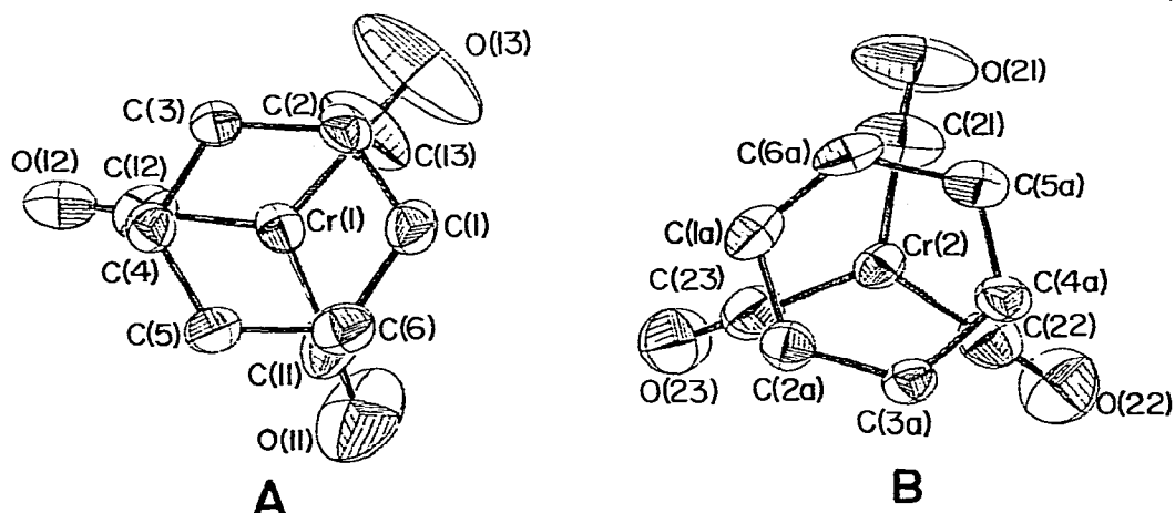
Fig. 2. Fragments of the molecule projected down the centre of the ring—chromium axis and showing the orientation of the \text{M}(\text{CO})_3 fragment. A, ring \text{C}(i) ( i = 1-6 )— \text{Cr}(1) ; B, ring \text{C}(ia) ( i = 1-6 )— \text{Cr}(2) .
